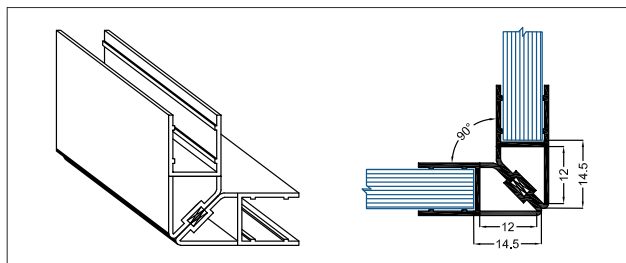
TPS-M3-PVC ₹ 1,100 90° Magnetic Seal
