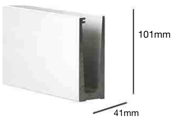
TCL-01 ₹ 7,000/mtr Floor to Glass Clamp Length : 3mtr
