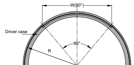
Convex Installation
