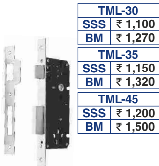
TML-30 (30x85mm) TML-35 (35x85mm) TML-45 (45x85mm) Lock Body for Wooden Doors with Latch & Dead Bolt
