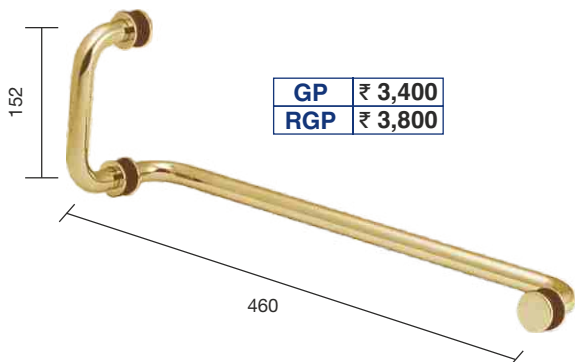
TGH-TB-1 GOLD Towel Bar with Handle (Ø19 mm)
