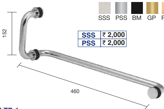
TGH-TB-1 Towel Bar with Handle (Ø19 mm)
