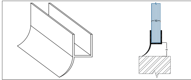
TPS-1 Wall Seal
