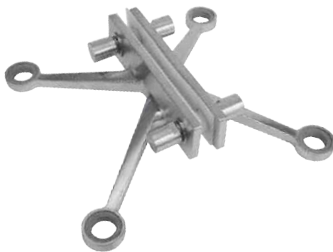
TSP-A4 Four Way Spider with Fin
