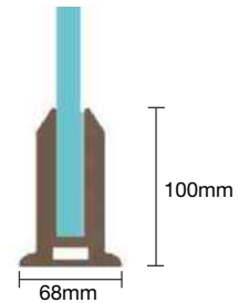
TBF-SG-AL-4 ₹ 2,350 Floor to Glass Clamp Length 70mm
