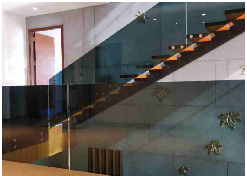
TRF-GC-01 Round Glass Clamp for Flat Surface
