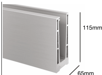
TCL-02 ₹ 10,000/mtr Floor to Glass Clamp Length : 3mtr
