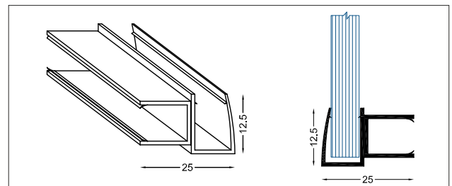
TPS-SL-BR-11-PVC ₹ 820 Brush Seal (Sliding Door)
