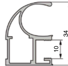
TWS-HP1 Handle Profile for Frame
