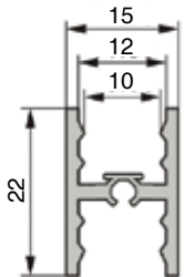
TWS-MP Middle Profile for frame
