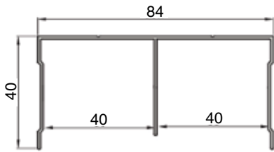
TWS-TT Double top track
