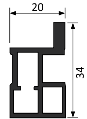
TWS-HP2 Handle Profile for Frame
