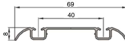
TWS-BT Double Bottom track
