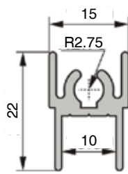
TWS-TP Top Profile for Frame
