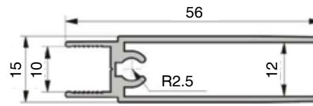
TWS-BP Bottom Profile for frame
