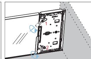
Turn screw driver to release lock 1, then release lock 2, remove the drawer front
