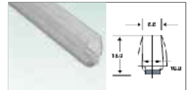
OPS-SL-BR-11 10mm STD ₹868 OPS-SL-BR-11 12mm STD ₹1,029 Brush Seal (Central)
