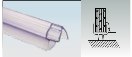
OPS-6 8MM STD ₹334 OPS-6 10MM STD ₹334 Water Dispersal Seal
