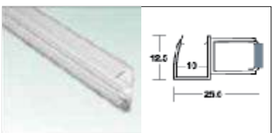
OPS-SL-BR-22-10ft 12m STD ₹1,029 OPS-SL-BR-22N-10ft 12mm ₹1,029 Weather Seal (Sliding Doors)
