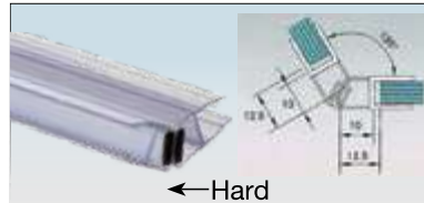
OPS-M2 8MM STD ₹1,202 OPS-M2 10MM STD ₹1,283 OPS-M2 8MM, 10MM, 12MM STD BM ₹1,382, ₹1,473, ₹1,474 135° Magnetic Seal
